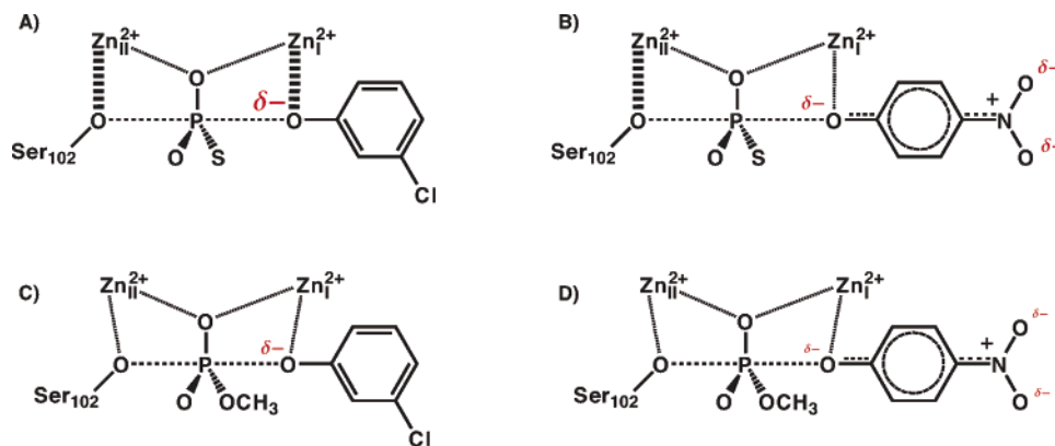
Figure 6. Resonance effects weaken interactions with active site Zn^{2+} for a loose transition but have a smaller effect on a tight transition state. (A) There is a large amount of charge buildup on the bridging oxygen in the transition state for hydrolysis of phenyl phosphorothioates (3-chlorophenyl phosphorothioate is arbitrarily chosen as an example). (B) 4-Nitro and 4-cyano groups delocalize electron density buildup at the bridging oxygen and weaken the interaction with the active site Zn^{2+} , leading to a smaller than expected overall rate enhancement. (C) In the tighter transition state for the phosphate diester hydrolysis reaction, there is less charge buildup at the bridging oxygen. Interactions with Zn^{2+} may be weaker and therefore less important for the rate enhancement. (D) 4-Nitro and 4-cyano groups delocalize charge, but if the interaction with Zn^{2+} is weaker, the deviation from the expected rate enhancement will be smaller.
