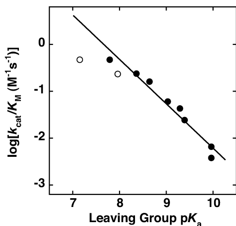
Figure 4. R166S AP-catalyzed hydrolysis of methyl phenyl phosphate diesters. Values of k_{\text{cat}}/K_{\text{M}} ( \text{M}^{-1} \text{s}^{-1} ) are from Table 1. The solid line is a least-squares fit to the data with a slope ( \beta_{\text{lg}} ) of -0.95 \pm 0.08 . Rate constants for compounds with 4-nitrophenyl and 4-cyano substituents (open circles) were omitted from the fit based on previous results with phosphorothioate and sulfate esters in which leaving groups with these substituents were unambiguous outliers. 24,26,28
