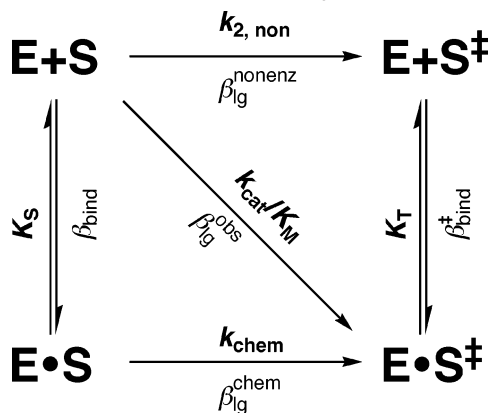
Scheme 4. Binding Interactions Affect \beta_{lg}
