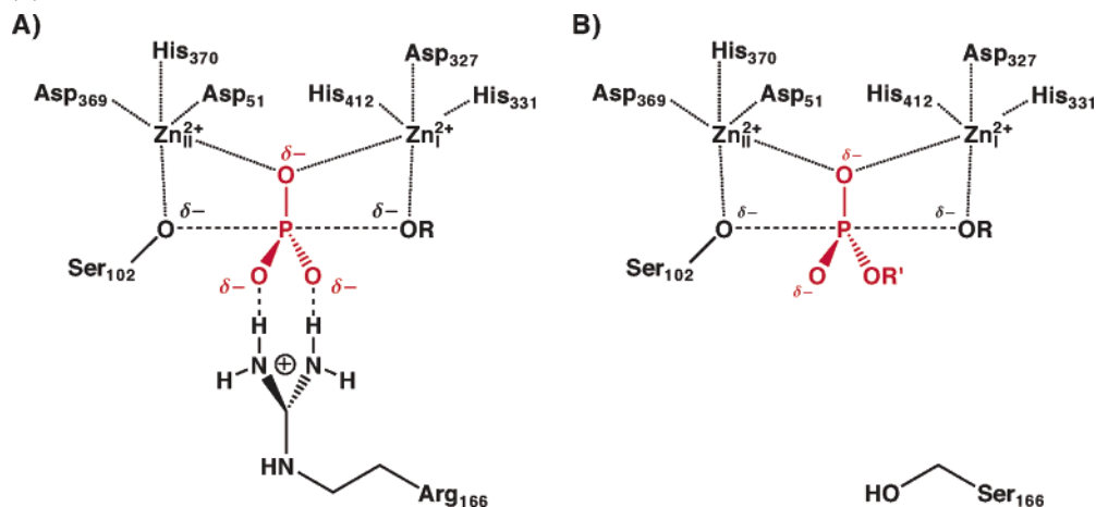
Scheme 1. Proposed AP Active Site Interactions of wt AP with a Phosphate Monoester Substrate (A) and of R166S AP with a Phosphate Diester Substrate (B) a 12,13
