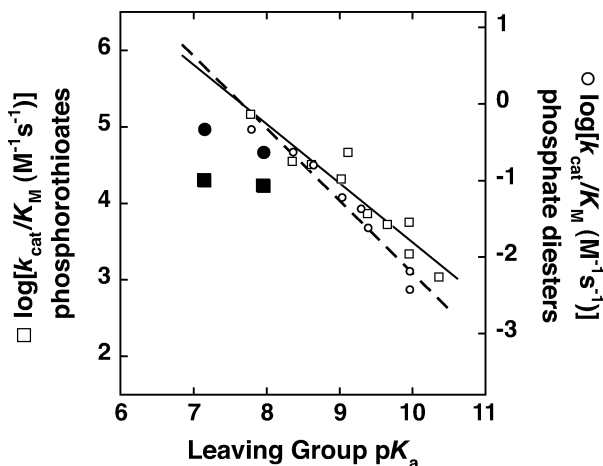
Figure 5. Deviations from the methyl phenyl phosphate diester LFER are small. LFERs for wt AP-catalyzed hydrolysis of phenyl phosphorothioates ( \square , \blacksquare ) 24 and R166S AP-catalyzed hydrolysis of methyl phenyl phosphate diesters ( \circ , \bullet ) are superimposed. The lines are least-squares fits to the data (open symbols) with a slope ( \beta_{lg} ) of -0.77 \pm 0.09 for phenyl phosphorothioates (solid line) and -0.95 \pm 0.08 for phosphate diesters (dotted line). Rate constants for compounds with 4-nitrophenyl and 4-cyano substituents (filled symbols) were not included in either fit. These leaving groups significantly deviate from the phosphorothioate LFER, but show smaller deviations from the diester LFER.
