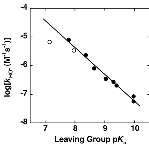
Figure 3. Leaving group dependence for attack of hydroxide ion on methyl phenyl phosphate diesters. Values of k_{\text{HO}^-} ( M^{-1} s^{-1} ) are from Table 1. The solid line is a least-squares fit to the data with a slope ( \beta_{\text{lg}} ) of -0.94 \pm 0.05 . Rate constants for compounds with 4-nitrophenyl and 4-cyano substituents (open circles) were omitted from the fit based on literature precedent for the occurrence of outliers due to resonance effects (see Supporting Information).
